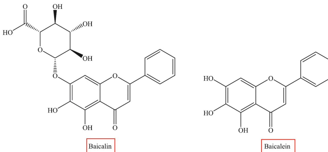
Figure 1. Structures of baicalein and baicalin.
